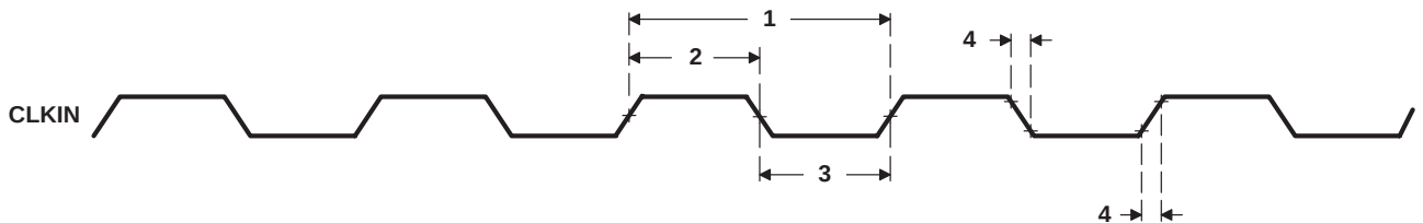
Figure 22. CLKIN Timings
