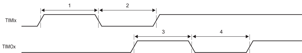
Figure 7-58 Timer Timing
