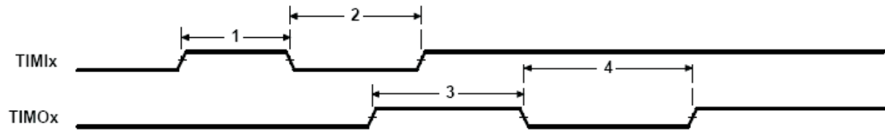
Figure 7-42. Timer Timing
