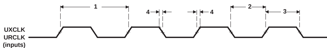
Figure 7-62. UTOPIA Clock
