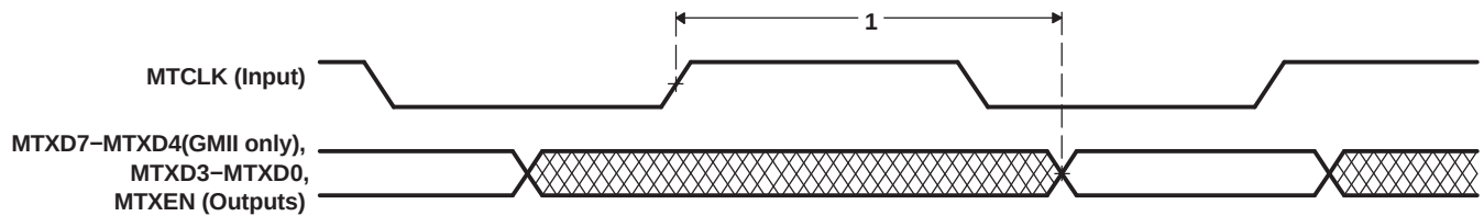
Figure 7-63. EMAC Transmit Interface Timing [MI and GMII Operation]
