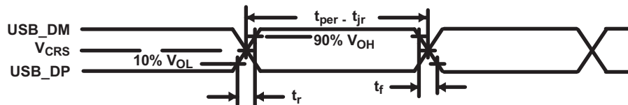
Figure 6-36. USB2.0 Integrated Transceiver Interface Timing
