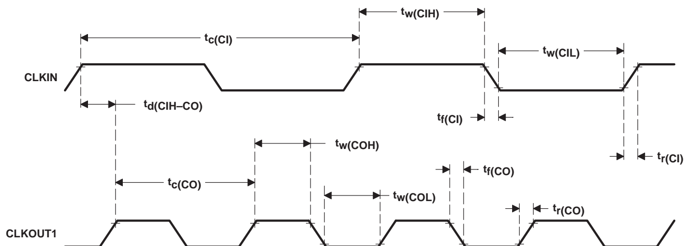
Figure 25. CLKIN-to-CLKOUT1 Timing With PLL (using \times 2 clock option) for TMS320C209
