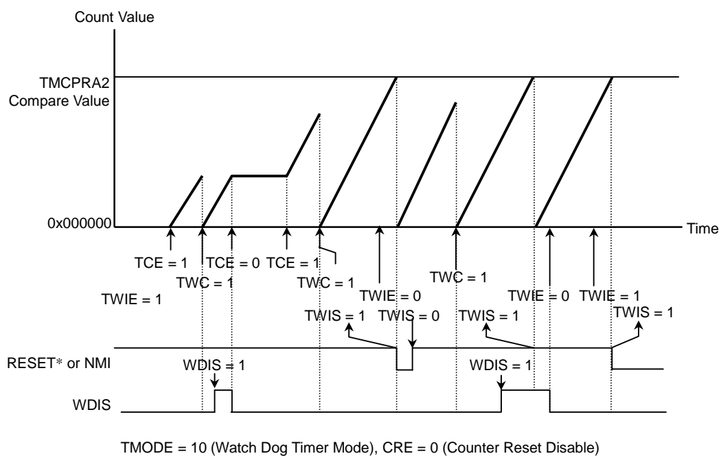
Figure 12.3.4 Operation Example of the Watchdog Timer Mode
