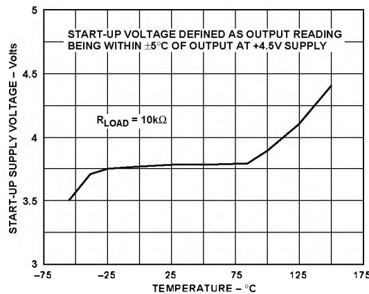
Figure 18. Start-Up Voltage vs. Temperature
