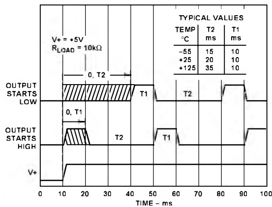
Figure 16. Start-Up Response
