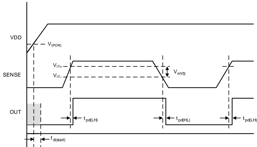
Figure 1. Timing Diagram
