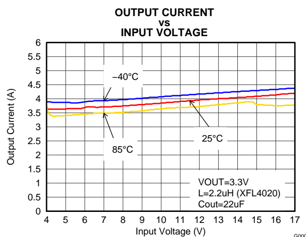
Figure 25. Maximum Output Current
