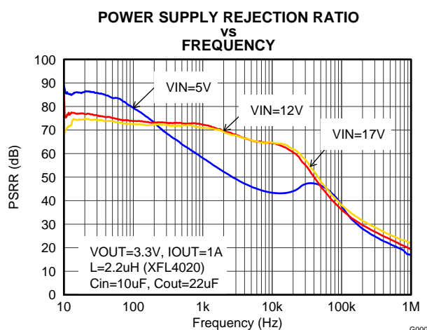
Figure 26. Power Supply Rejection Ratio, f_{SW}=2.5MHz
