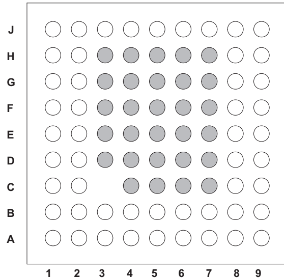
5x5mm 80-Ball BGA Package (Bottom View)
