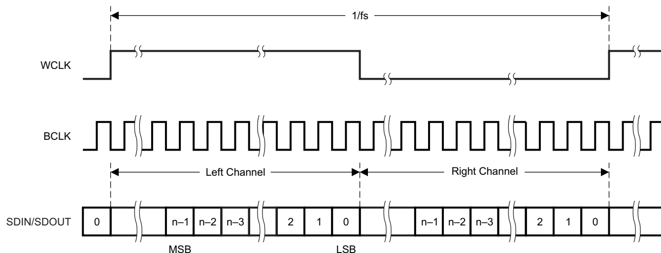
Figure 18. Right-Justified Serial Data Bus Mode Operation
