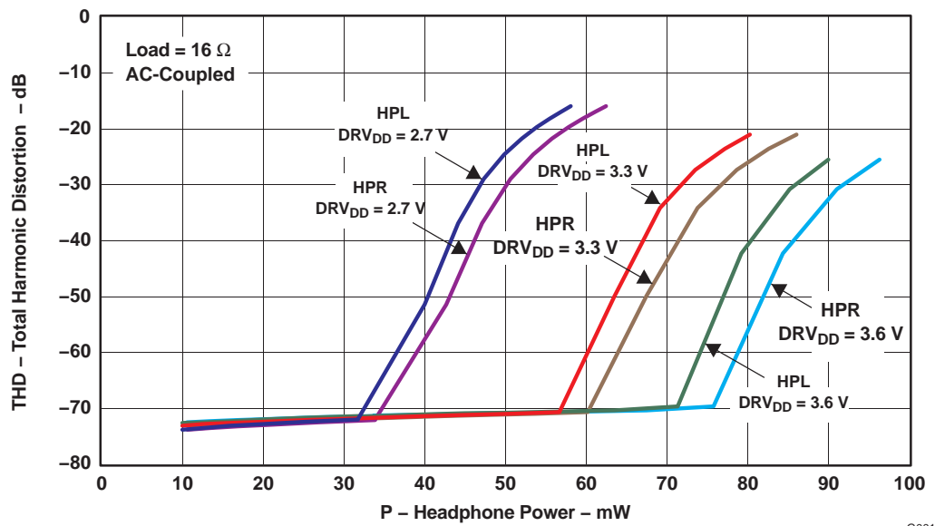
Figure 5. THD vs Headphone Power, 16-Ω Load
