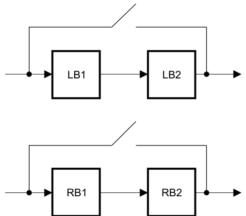
Figure 26. Structure of Digital Effects Processing for Independent Channel Processing
