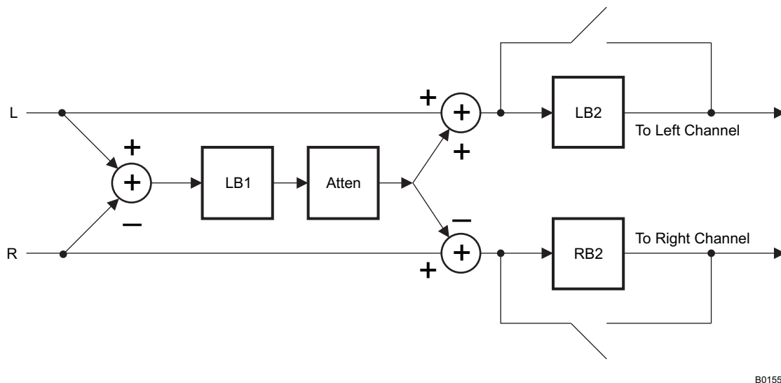
Figure 27. Architecture of the Digital Audio Processing When 3-D Effects Are Enabled
