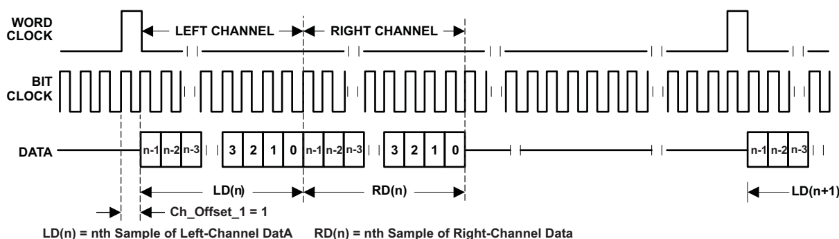
Figure 27. DSP Mode With Ch_Offset_1 = 1
