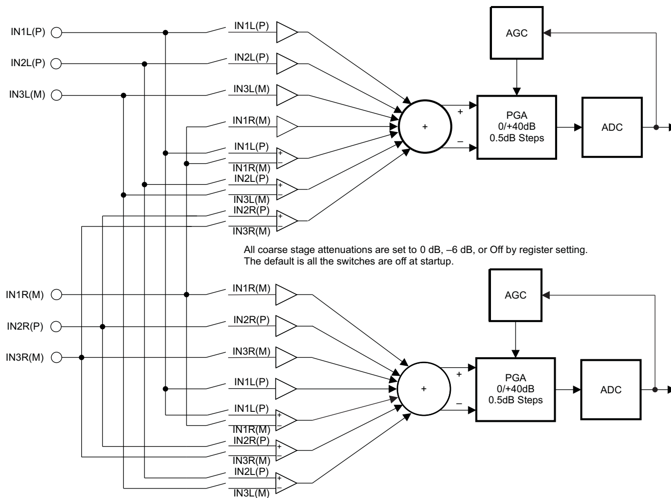
Figure 33. TLV320ADC3101 Available Audio Input Path Configurations
