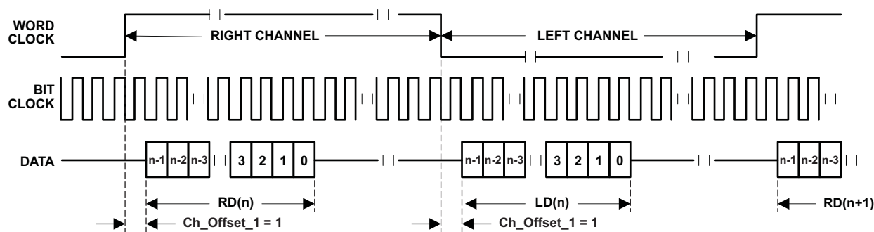
Figure 20. Left-Justified Mode With \text{Ch\_Offset}_1 = 1 , Channel Swapping Enabled
