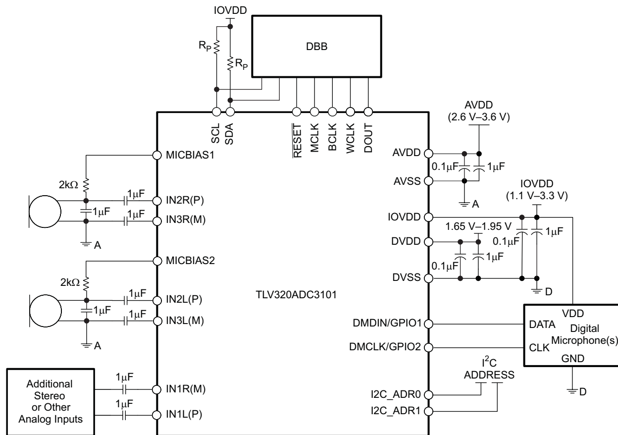
Figure 11. Typical Connections
