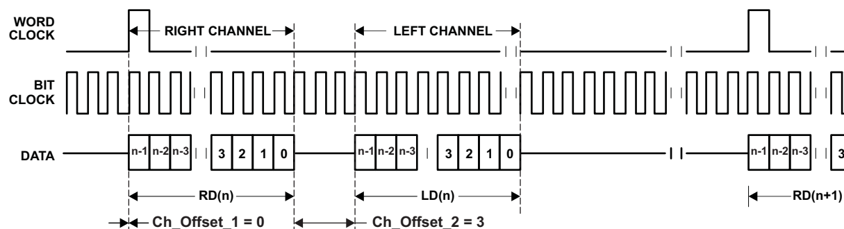
Figure 29. DSP Mode, Time-Slot-Based Mode Enabled, \text{Ch\_Offset}_1 = 0 , \text{Ch\_Offset}_2 = 3
