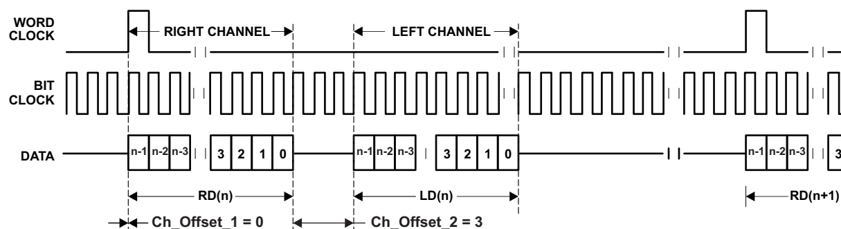
Figure 30. DSP Mode, Time-Slot-Based Mode Enabled, \text{Ch\_Offset}_1 = 0 , \text{Ch\_Offset}_2 = 3 , Channel Swap Enabled
