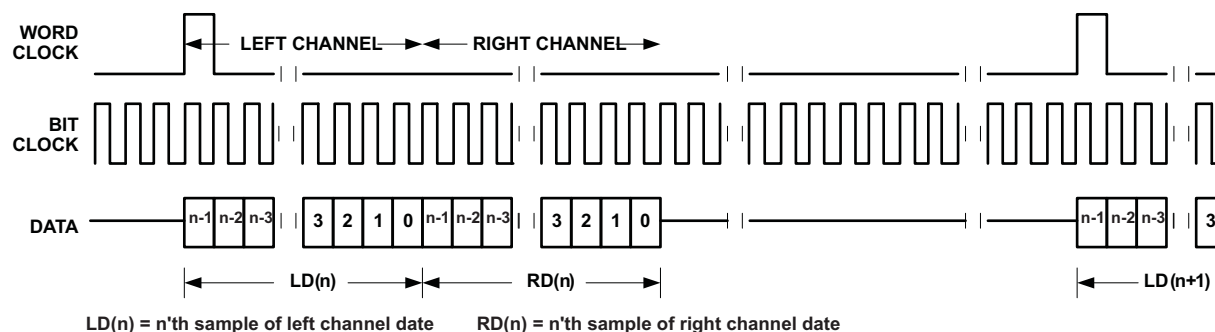
Figure 26. DSP Mode (Standard Timing)
