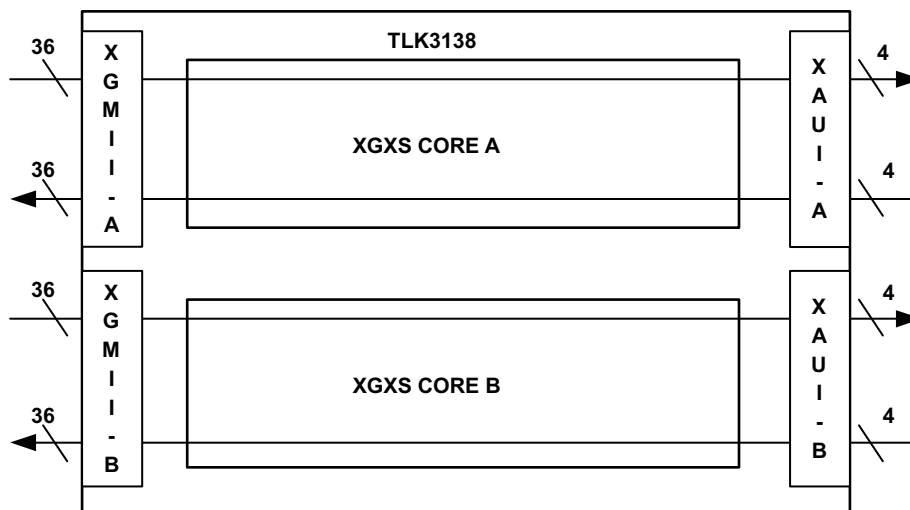
Figure 3. DUAL XAUI Application
