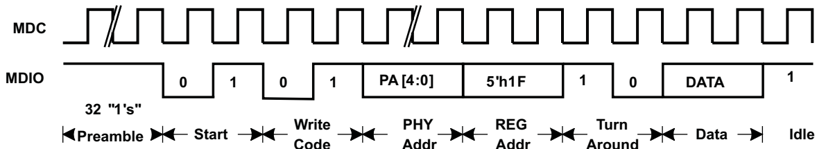
Figure 2-39. CL22 – Indirect Address Method – Data Write
