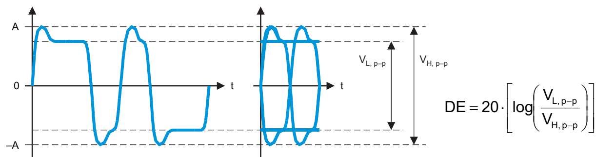
Figure 3. Output De-emphasis
