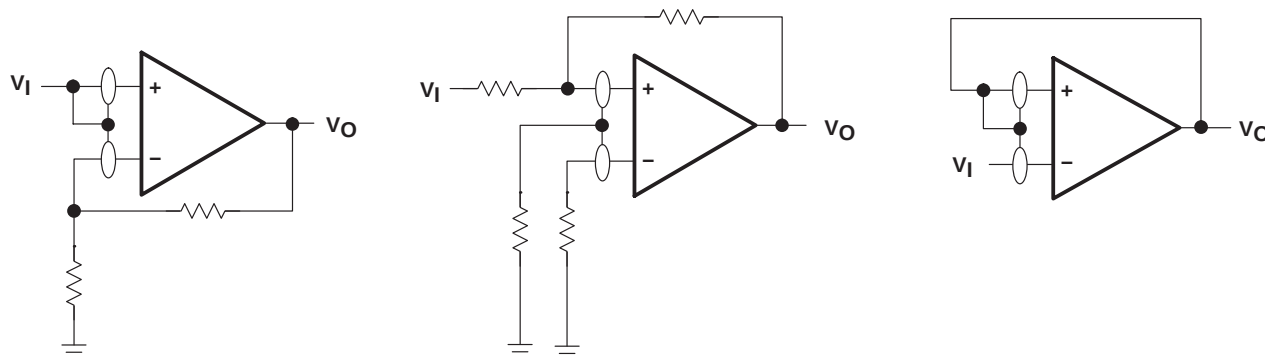
Figure 70. Use of Guard Rings
