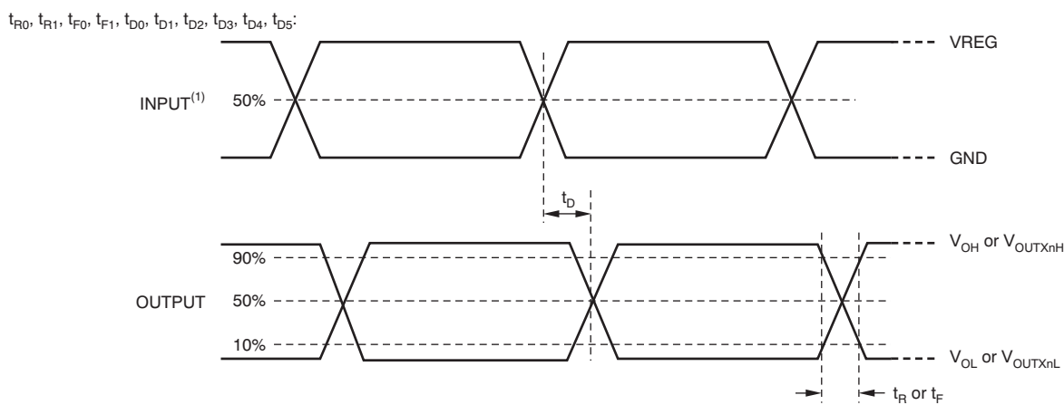
Figure 8. Output Timing
