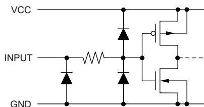
Figure 1. SIN, SCLK, GSKL, XLAT, BLANK, MODE, XHALF
