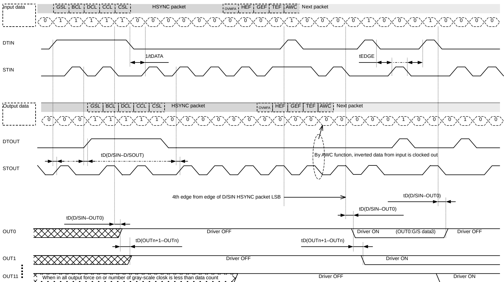
Timing chart 2 (when internal gray scale clock is used)
