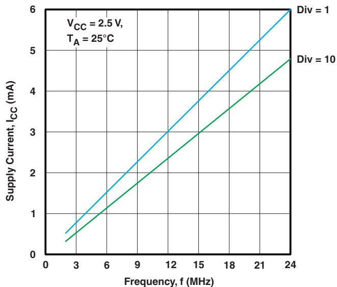
Figure 10. Supply Current vs Frequency ( V_{CC} = 2.5\text{ V} )
