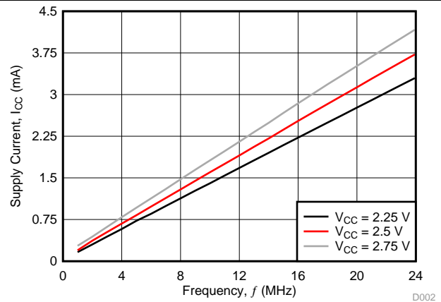
Figure 11. Supply Current vs Frequency ( V_{CC} = 2.25, 2.5, and 2.75\text{ V} )
