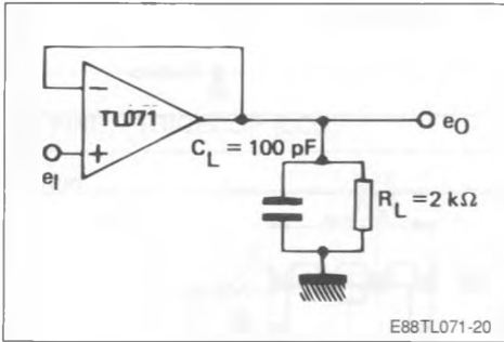
Figure 1 : Voltage follower.
