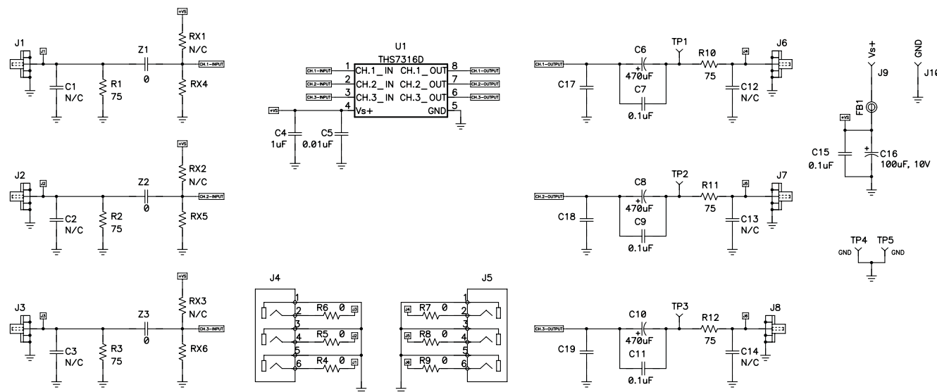
Figure 33. THS7316D EVM
