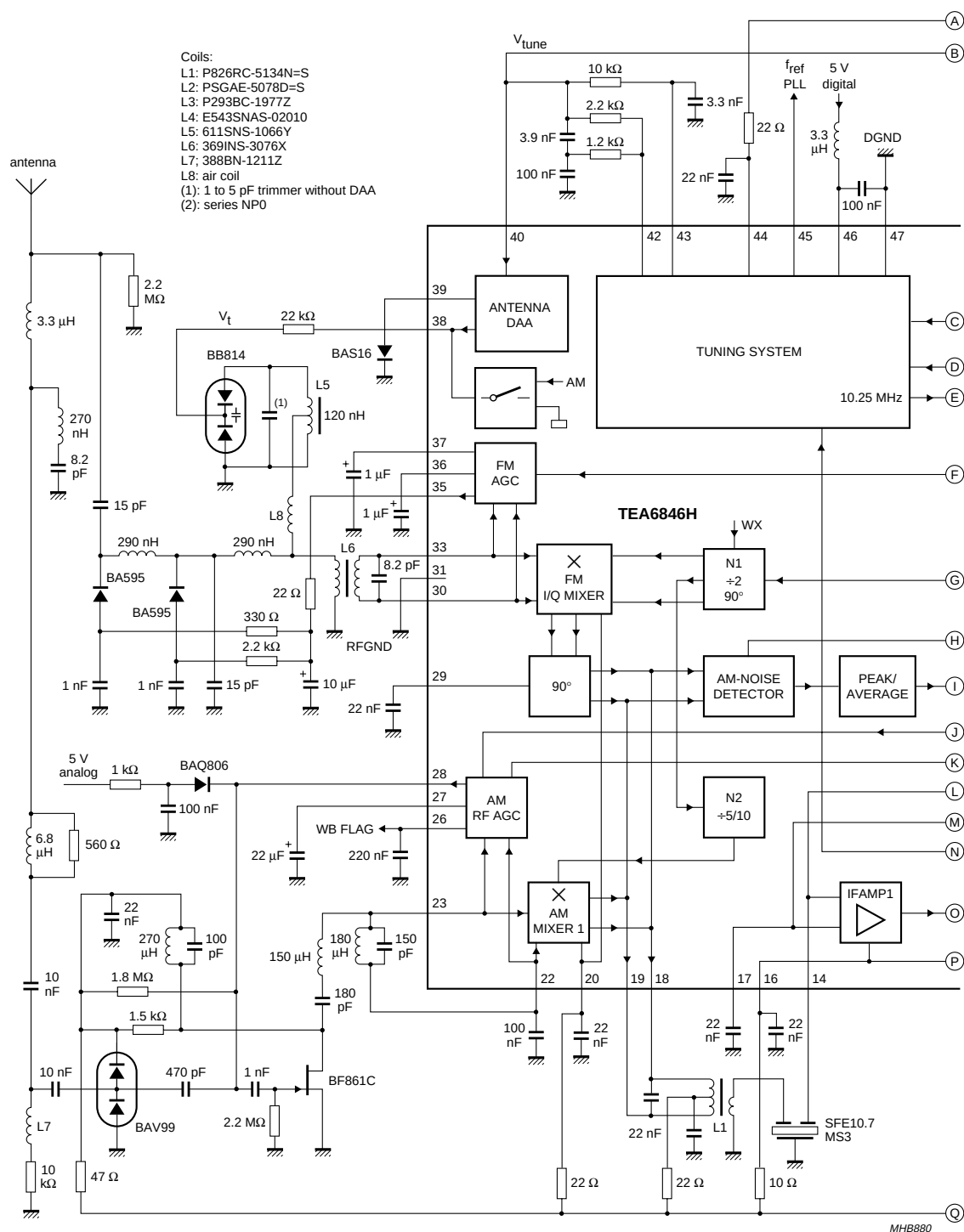
Fig.7 Application diagram (continued in Fig.8).
