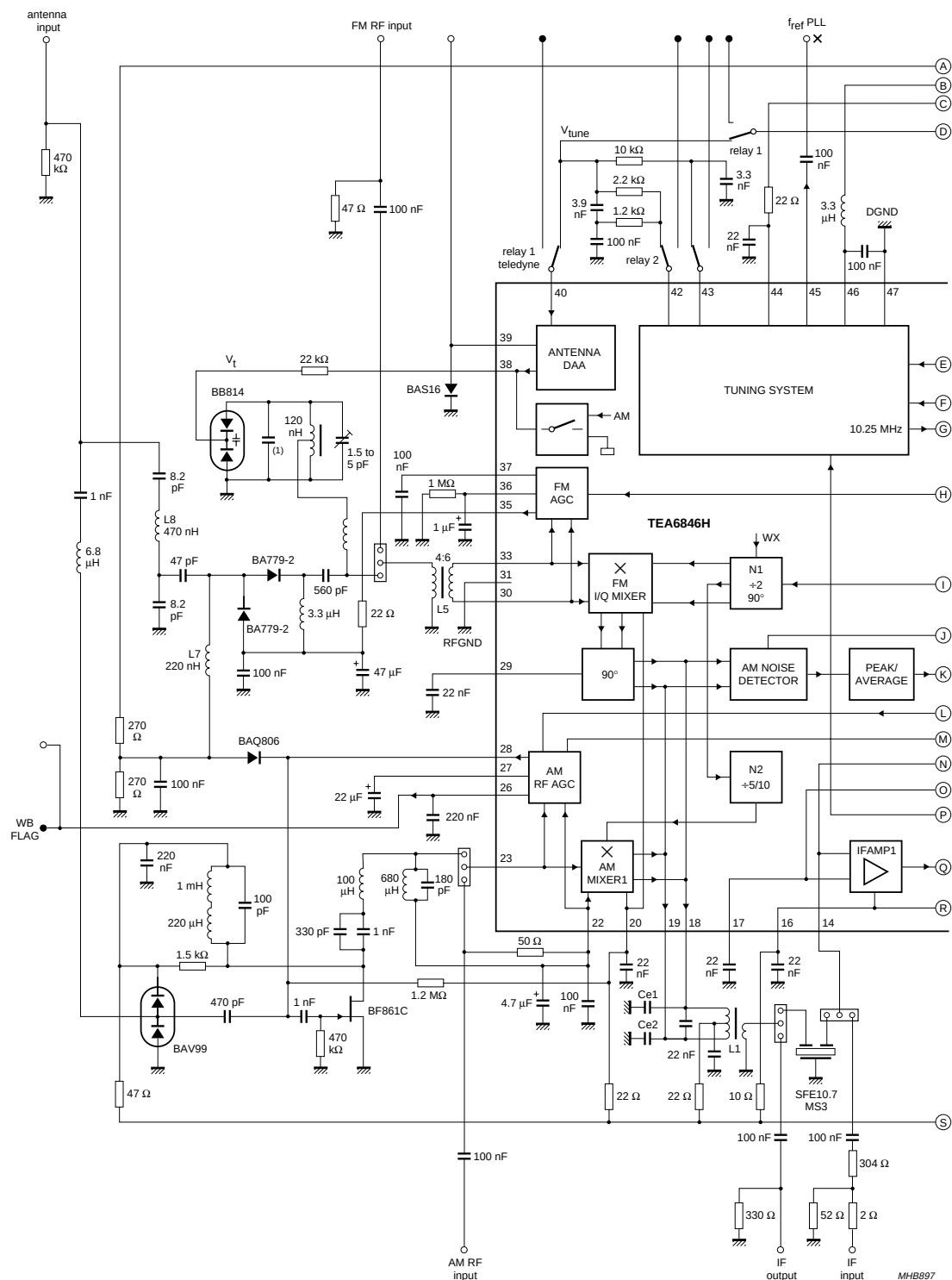
Fig.9 Test circuit (continued in Fig.10).
