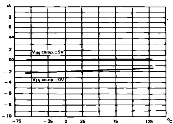
COMPARATOR INPUT CURRENT VS T_j and V_C
