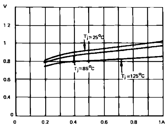
LOWER DIODE V_F VS I_{OUT} and T_j
