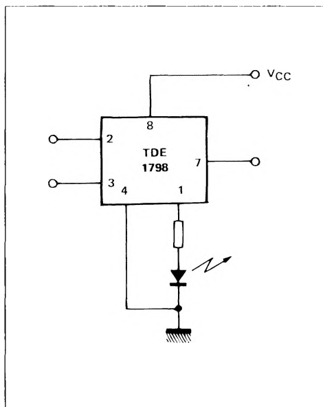
ALARM OUTPUT SOURCE
