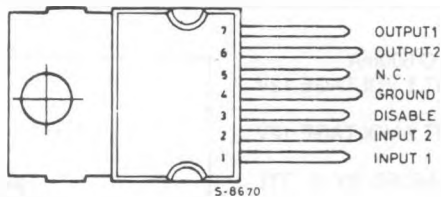
Tab connected to pin 4.
