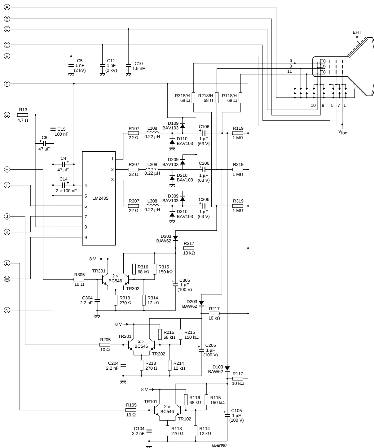
Fig.21 Application board with LM2435 (drawing continued from Fig. 20).
