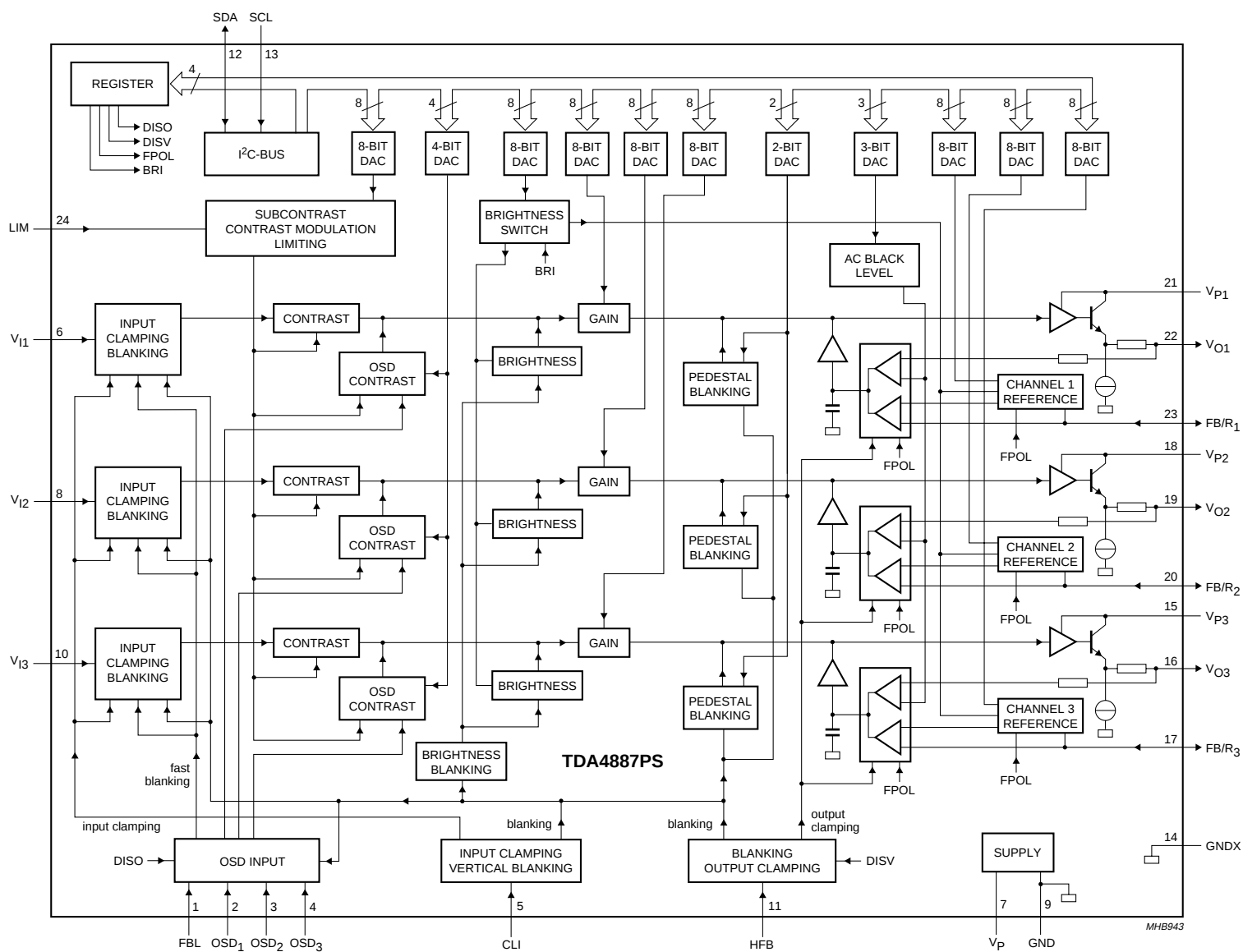
Fig.1 Block diagram.
