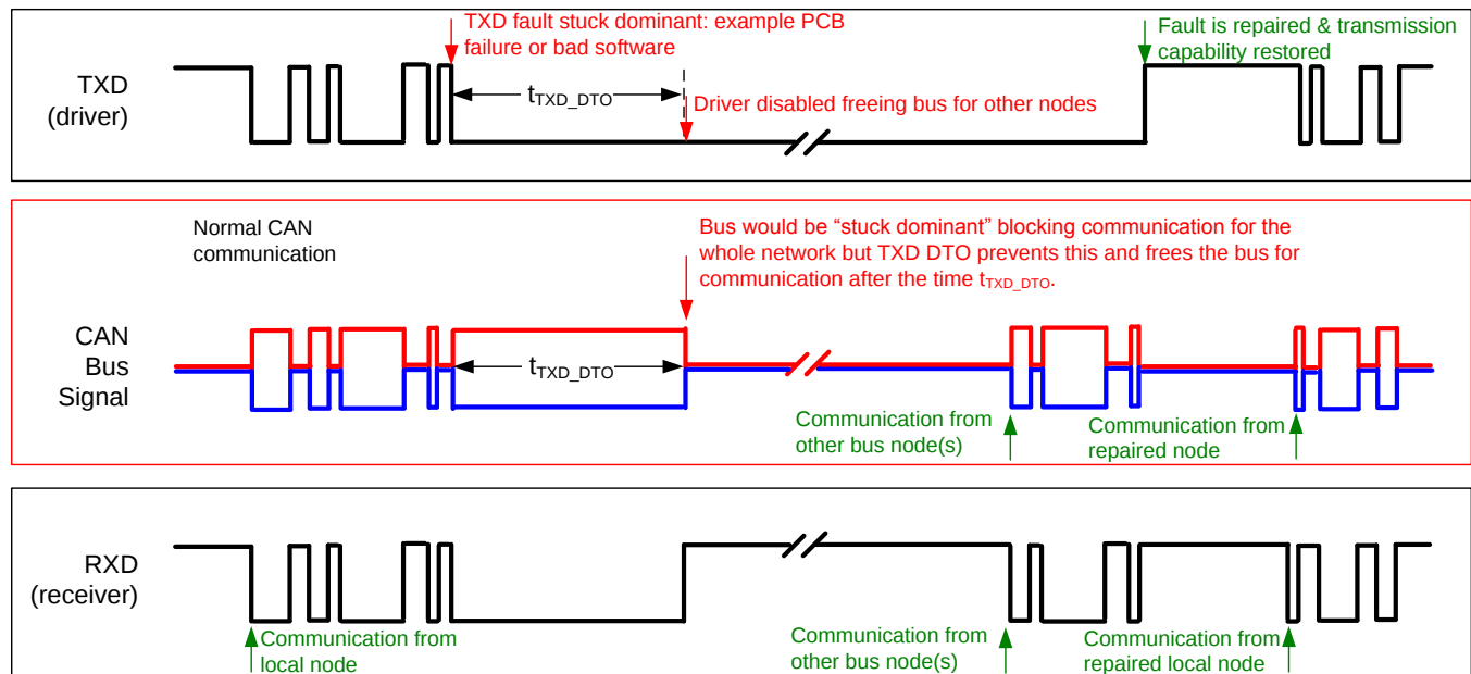
Figure 18. Example Timing Diagram for TXD DTO
