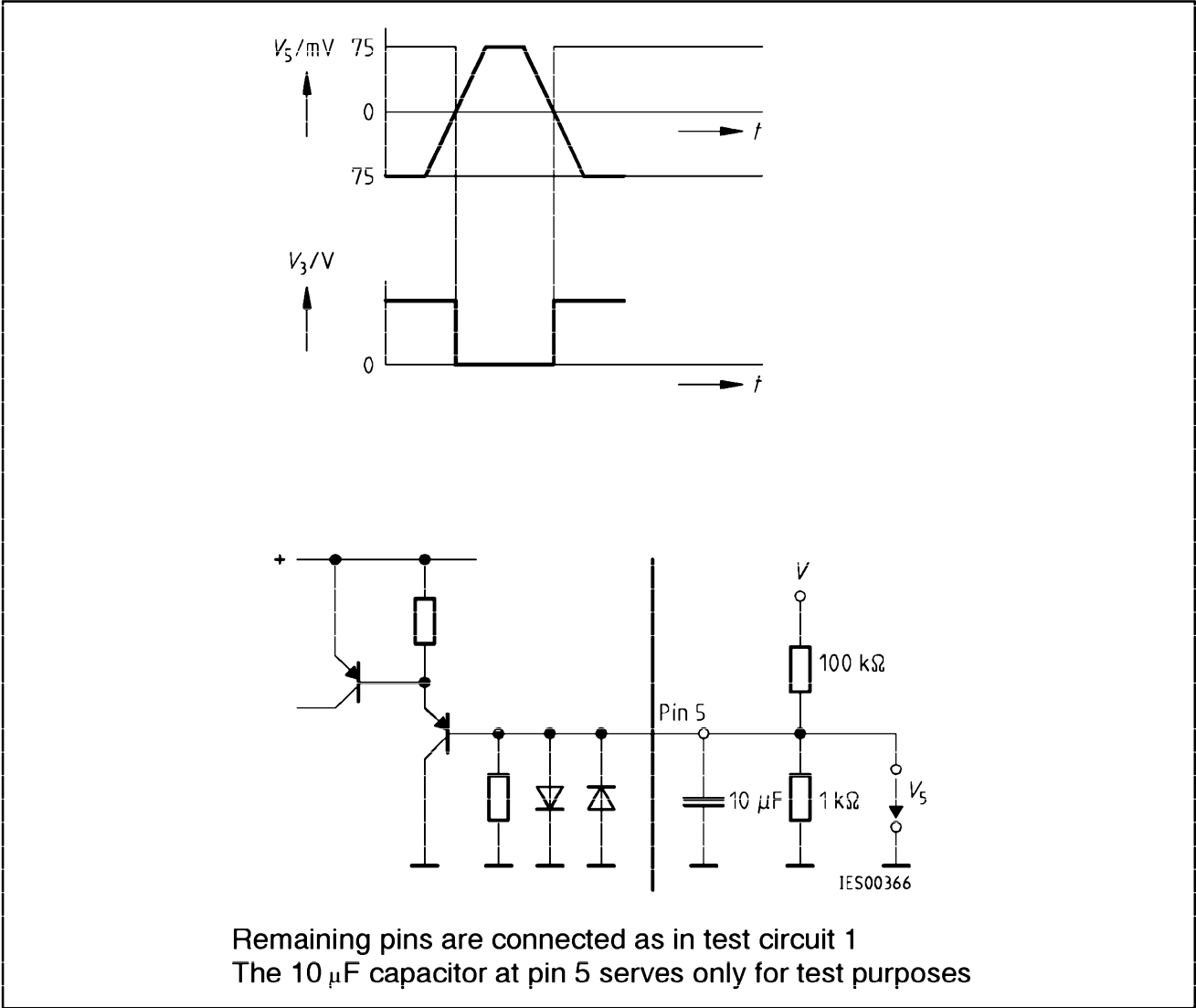
Test Circuit 4
