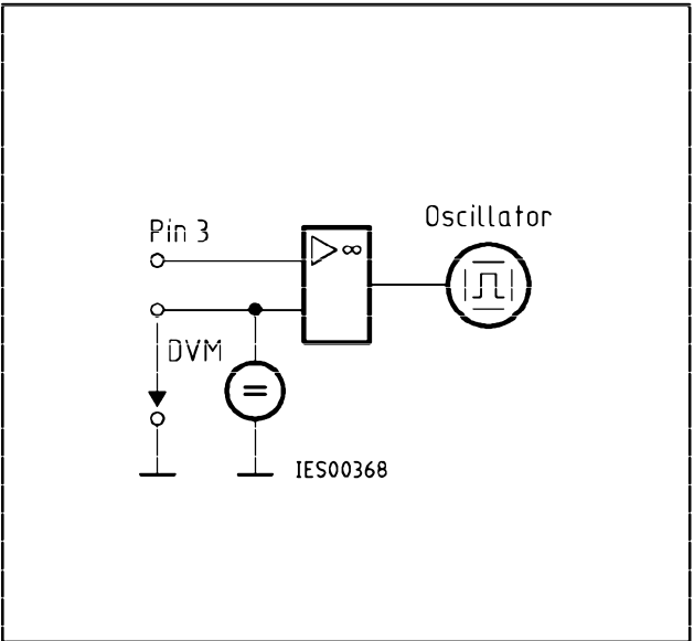
Test Circuit 6
