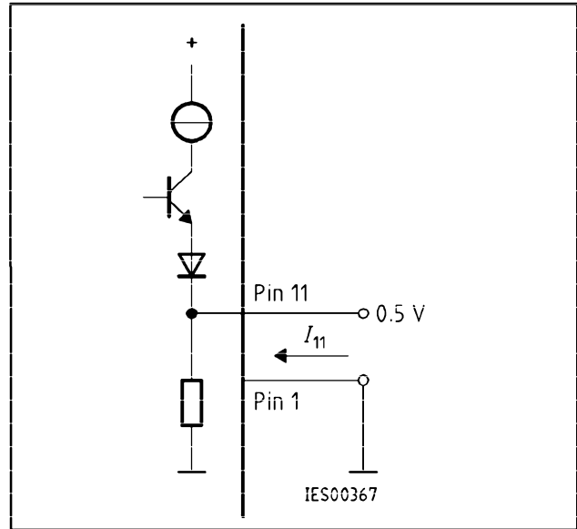
Test Circuit 5
