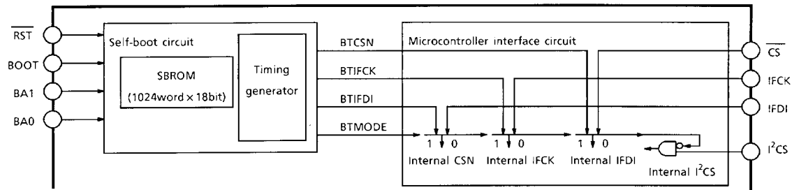
Figure 1 Self-boot system
