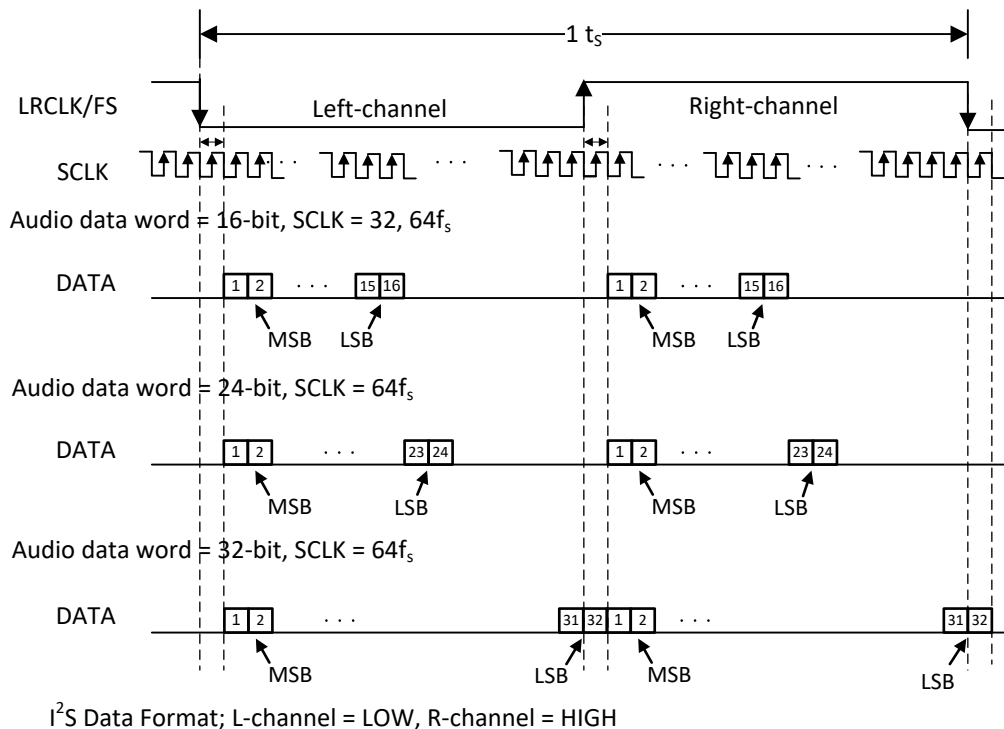
Figure 57. I²S Audio Data Format
