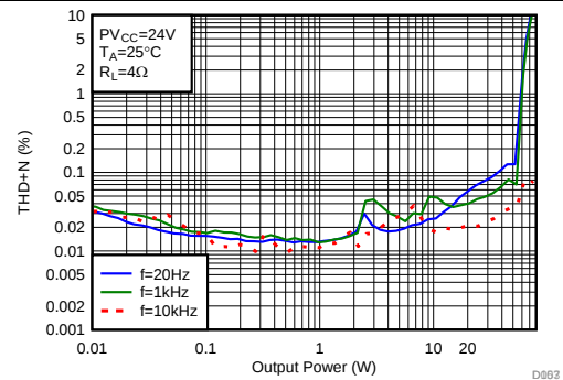
Figure 49. THD+N vs Output Power-PBTL
