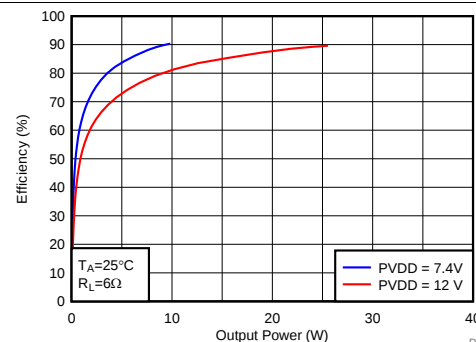
Figure 39. Efficiency vs Output Power-BTL
