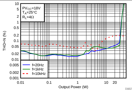
Figure 48. THD+N vs Output Power-PBTL
