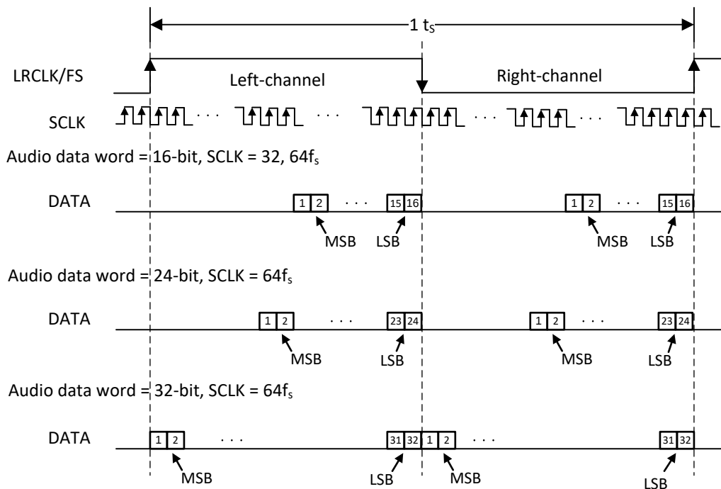
Figure 57. I²S Audio Data Format
