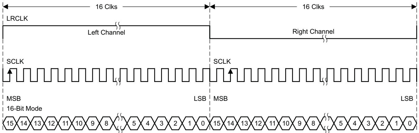
Figure 31. Left-Justified 32- f_s Format
