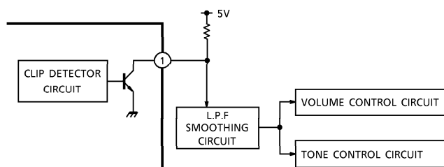
pin① : Open Collector Output (Active Low)
