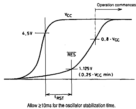
Figure 2. Reset time
