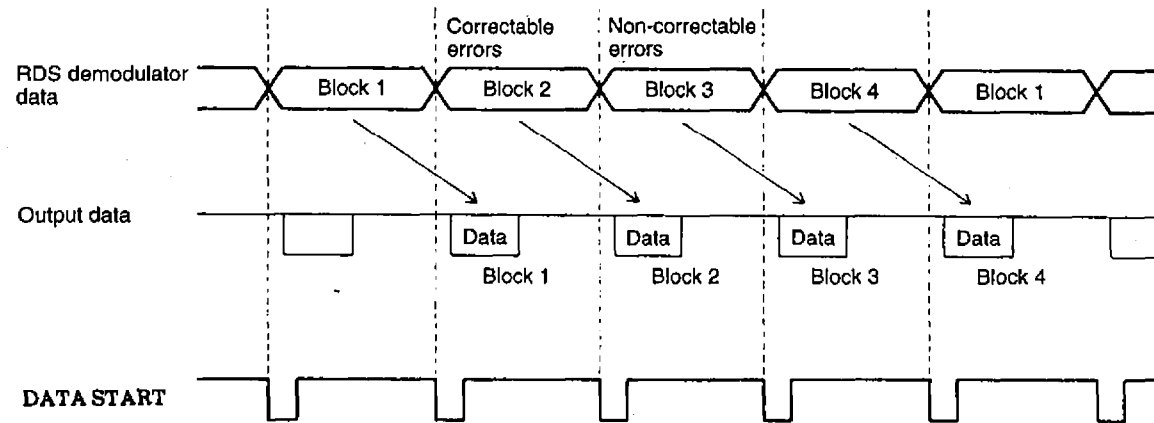
Figure 3. Demodulator data and output data relationship
