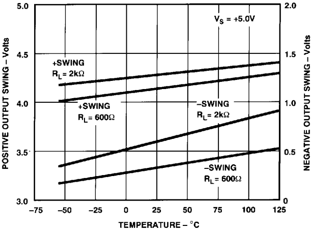
Figure 23. Output Swing vs. Temperature and Load
