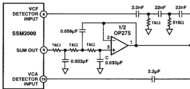
Figure 35. A Three-Pole Butterworth Filter
