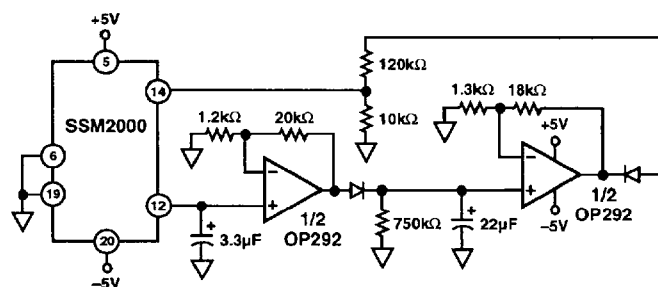
Figure 32. A Schematic to Use the SSM2000 in a Post-Volume Control Application
