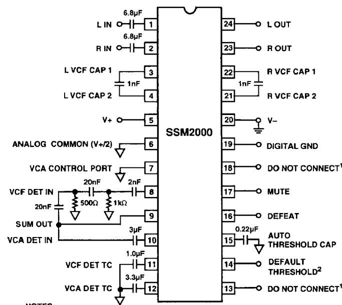
Figure 1. Typical Basic Application
