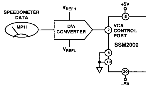
Figure 31. Volume Control vs. Road Speed Block Diagram
