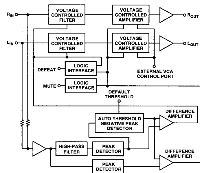
Figure 5. SSM2000 System Block Diagram
