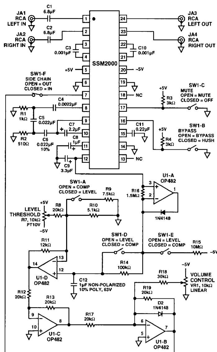
Figure 4. Typical Dual Supply Application and Test Circuit
