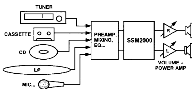
Figure 27. The Position of the SSM2000 in a Common Audio Signal Chain
