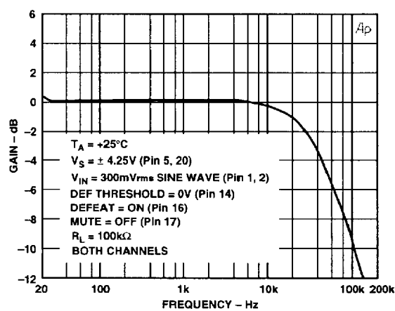
Figure 8. -3 dB Bandwidth
