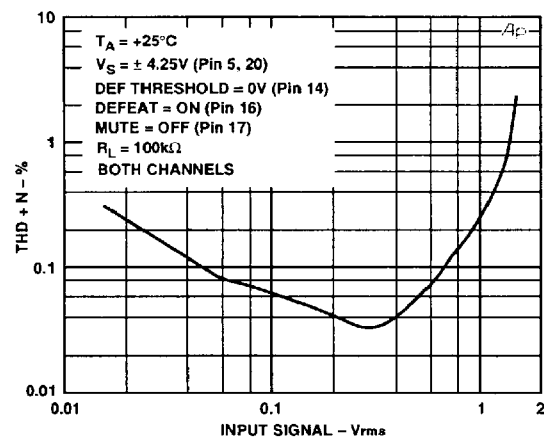
Figure 6. THD+N (%) vs. Input Signal
