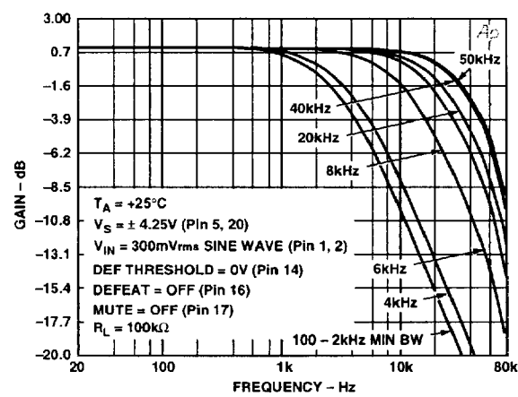
Figure 10b. VFC Characteristics (Simulated Noise Level 90 mV rms with Different Frequency) Applied through a 3-Pole HP filter
