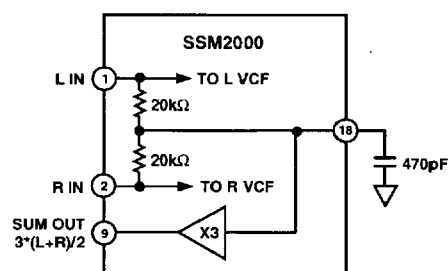
Figure 29. The Internal Circuit for SUM OUT
