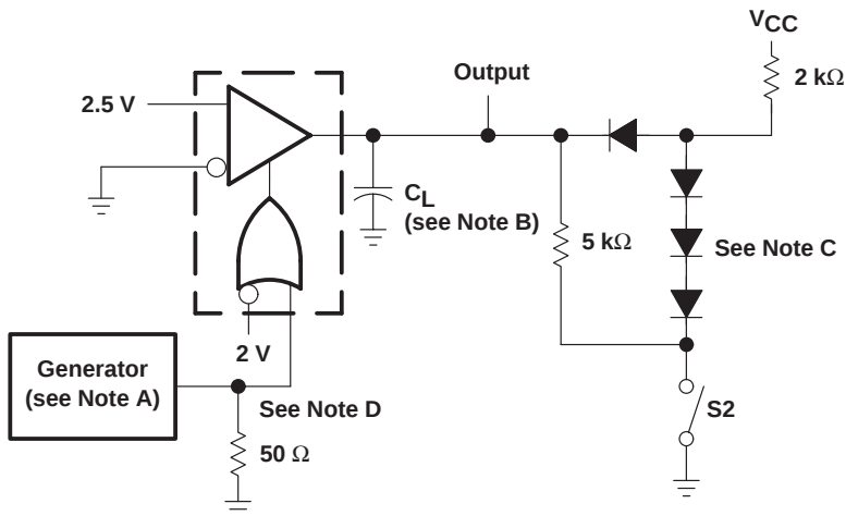
TEST CIRCUIT
