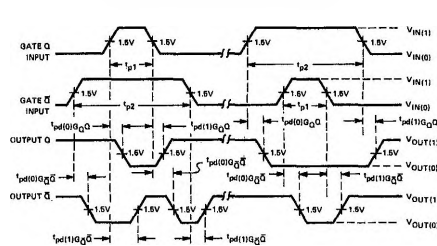
VOLTAGE WAVEFORMS
