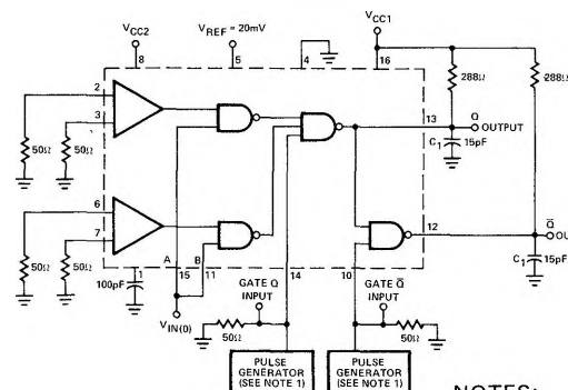
TEST CIRCUIT
