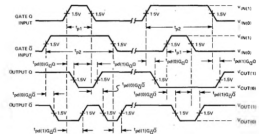
VOLTAGE WAVEFORMS
