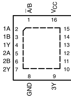
SN74AHC157 ... RGY PACKAGE (TOP VIEW)
