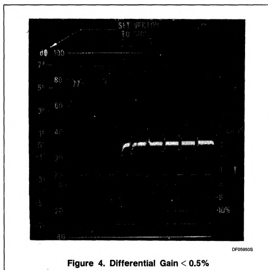
Figure 4. Differential Gain &lt; 0.5%
