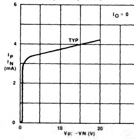
Supply Current per Op Amp
