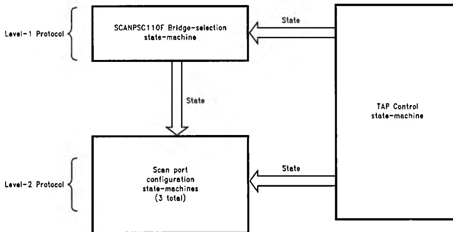
FIGURE 2. SCANPSC110F Bridge State Machines
