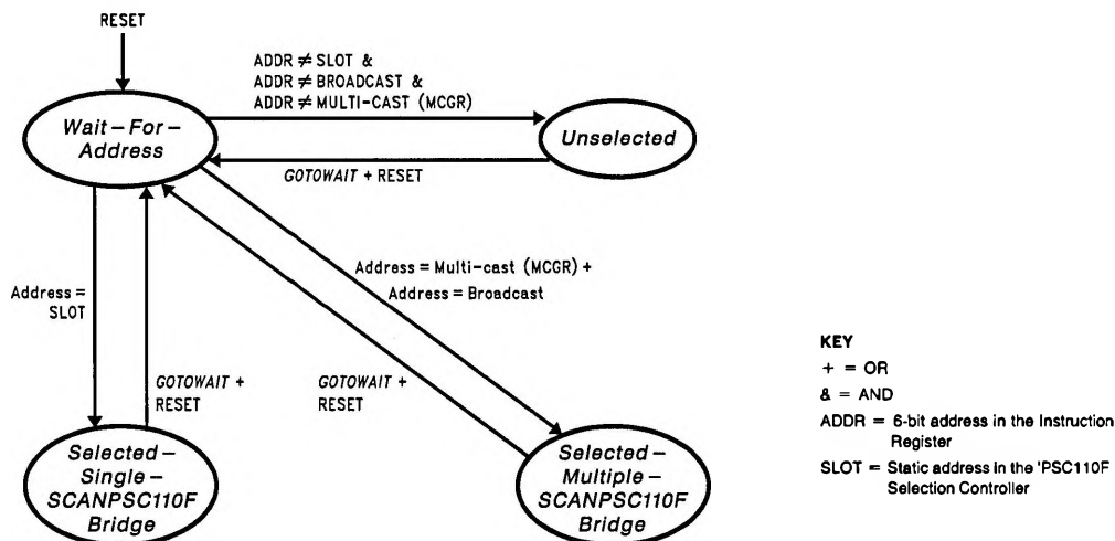
FIGURE 3. State Machine for SCANPSC110F Bridge Selection Controller
