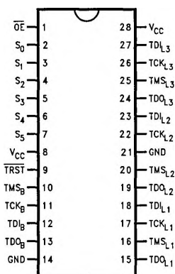
28-Pin SOIC, CDIP and Flatpak
