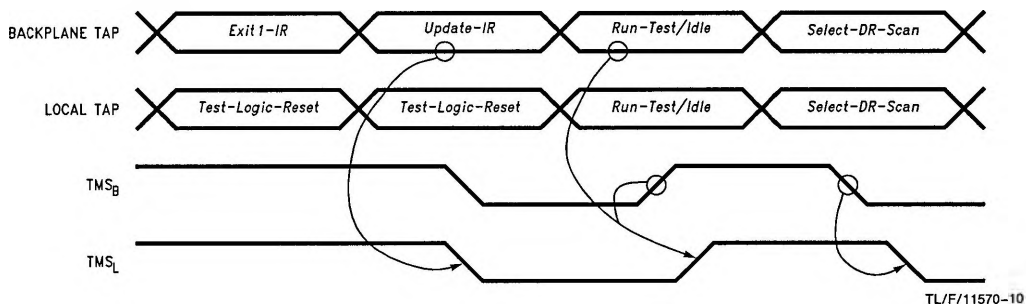
FIGURE 9. Local Scan Port Synchronization from Parked-TLR Instruction
