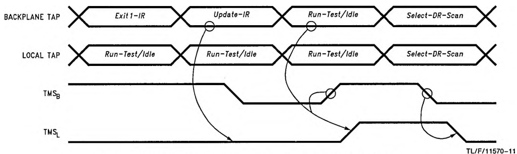
FIGURE 10. Local Scan Port Synchronization from Parked-RTI State
