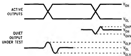
FIGURE 14. Quiet Output Noise Voltage Waveform
