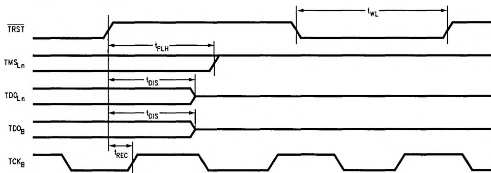
FIGURE 15. Reset Waveforms
