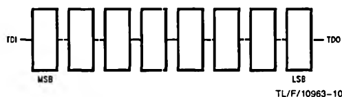
Instruction Register Scan Chain Definition
