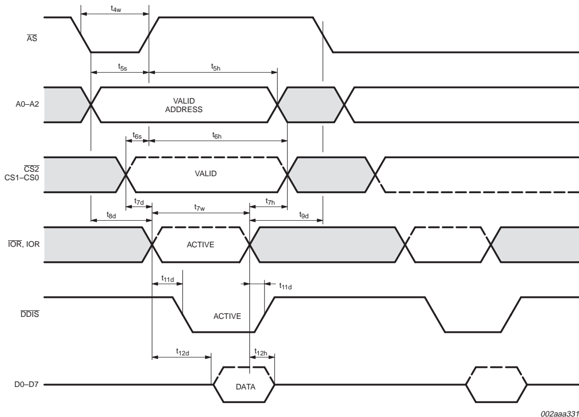
Fig 11. General read timing in 'standard' mode when using \overline{AS} signal.
