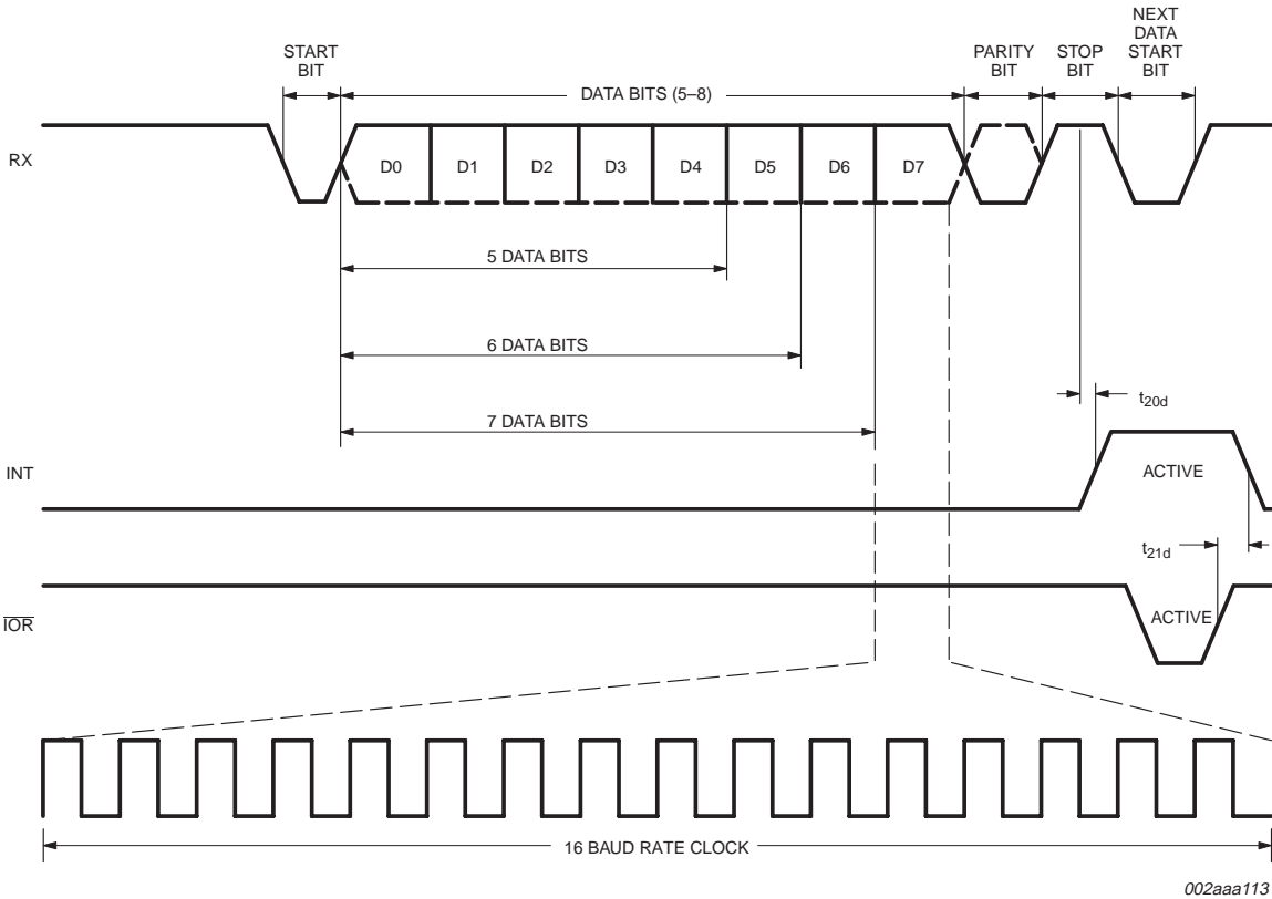
Fig 17. Receive timing.
