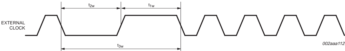
Fig 16. External clock timing.
