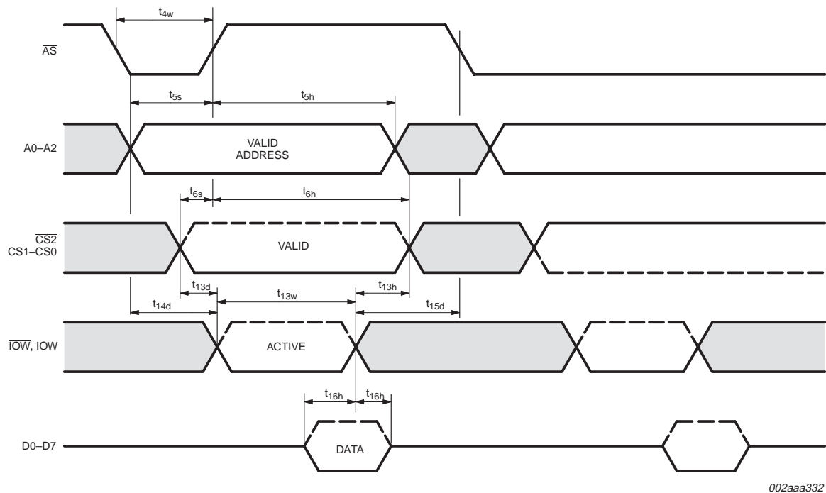
Fig 12. General write timing in 'standard' mode when using \overline{AS} signal.
