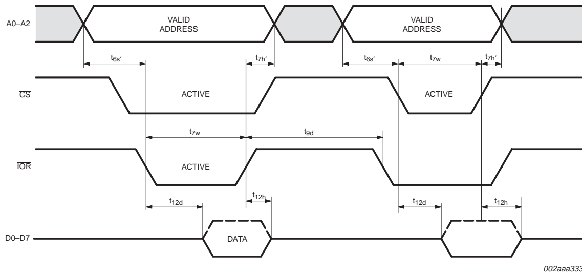
Fig 13. General read timing in 'standard' mode when \overline{AS} is tied to GND.
