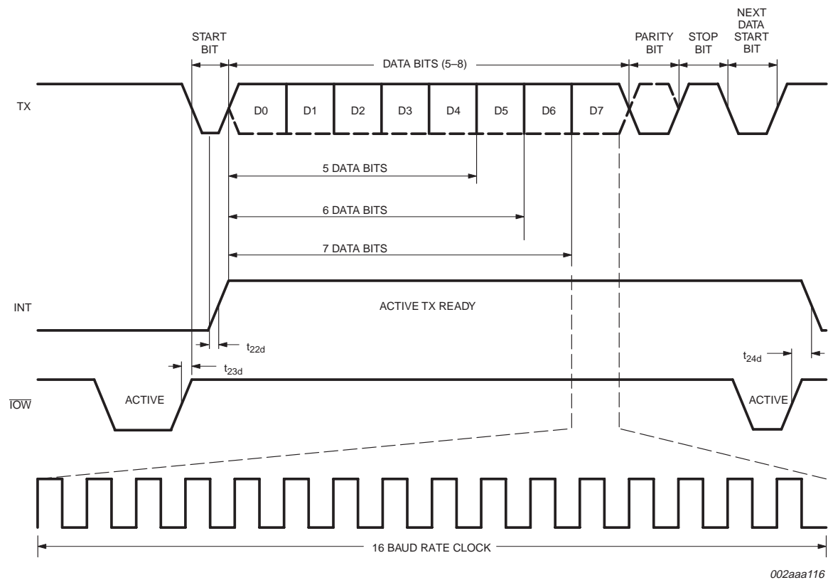
Fig 20. Transmit timing.
