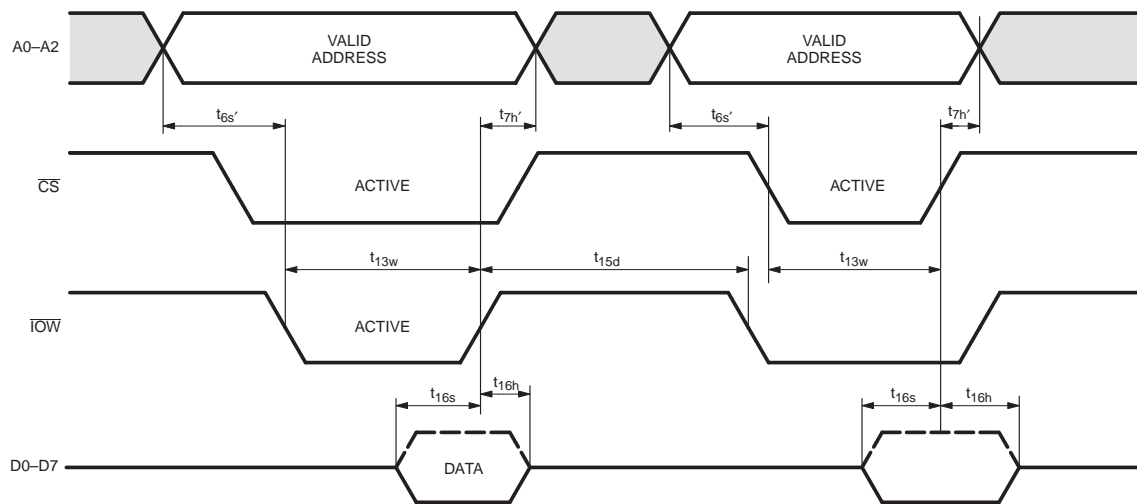
Fig 14. General write timing in 'standard' mode when \overline{AS} is tied to GND.
