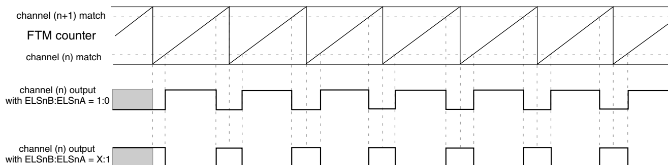
Figure 26-143. Combine mode
