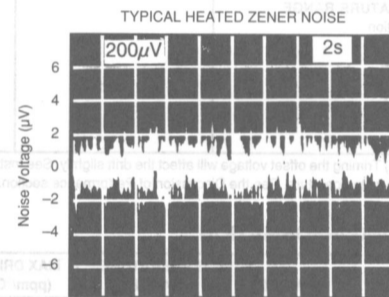
Low Frequency Noise (see Noise Test Circuit)
