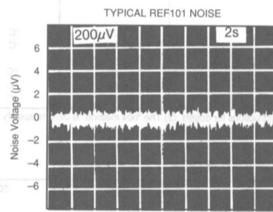
Low Frequency Noise (see Noise Test Circuit)
