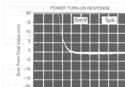
Power Turn-On
