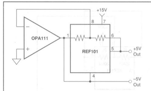
FIGURE 17. ±5V Reference.
